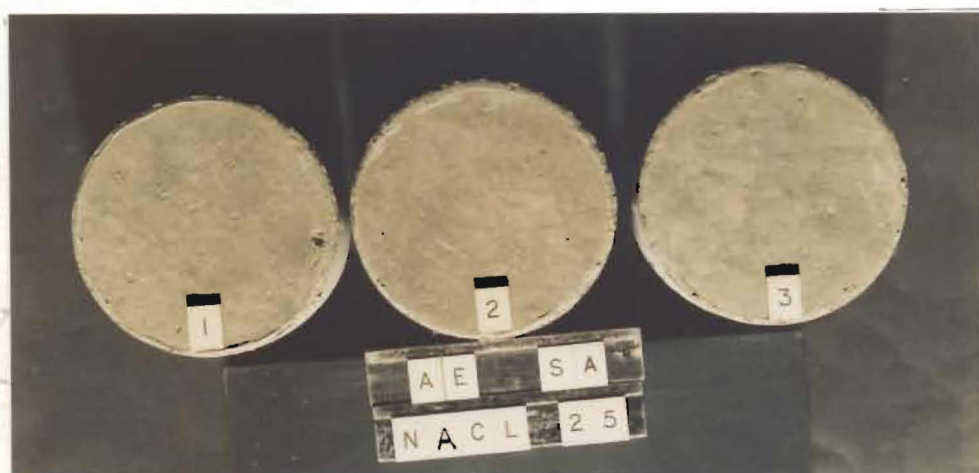
Sodium Chloride (25% solution) after 50 cycles
